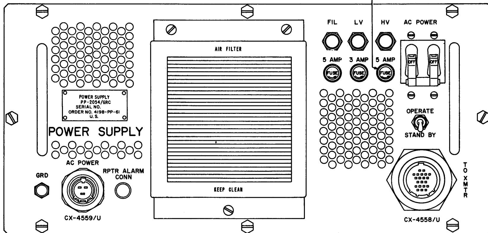
Figure 3-4. Power Supply PP-2054(*)/GRC, front panel view
