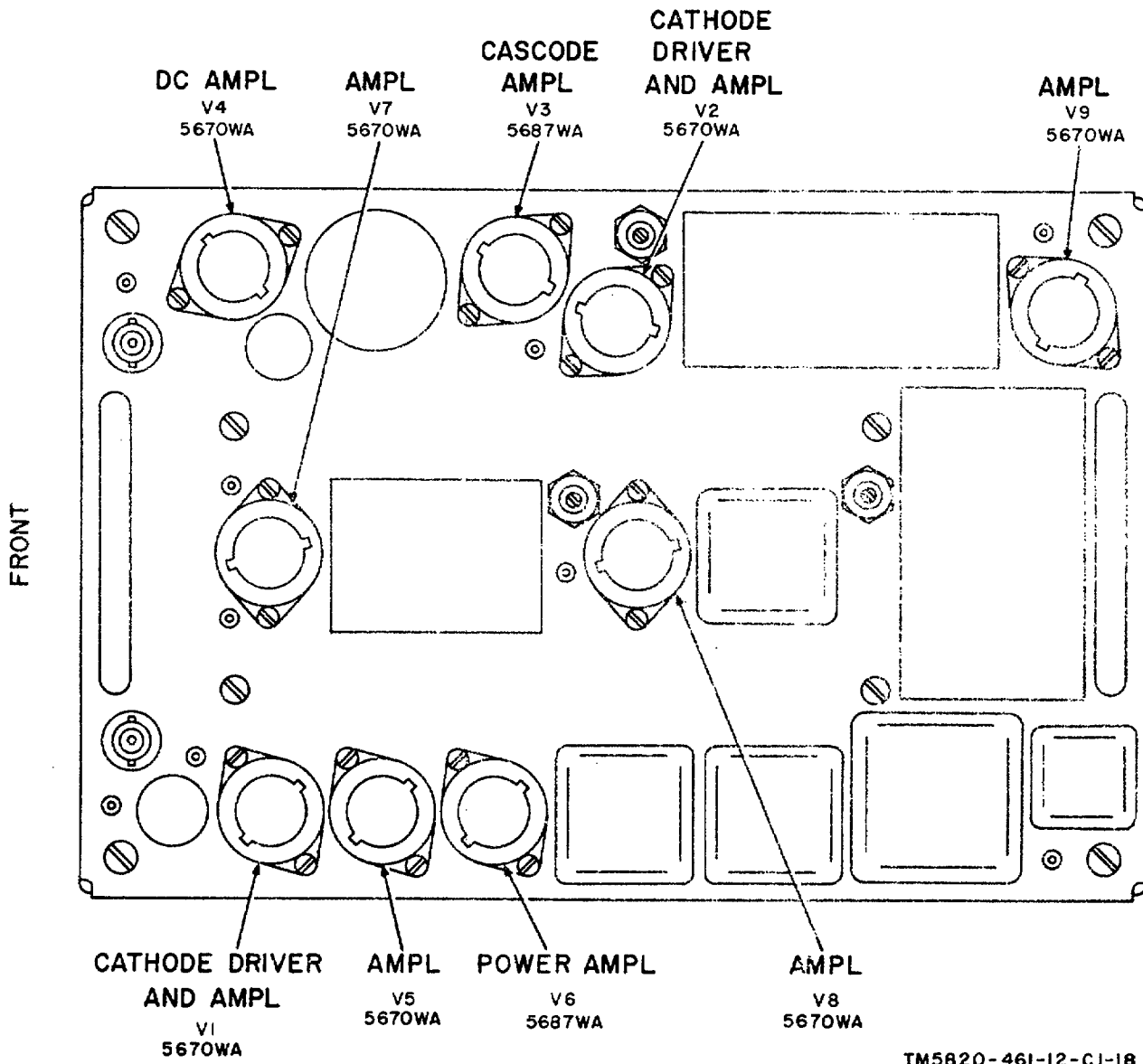
Figure 5-7. Baseband assembly 3A3 (part of R-1331(*) (P)/GRC or R-1148(P)/GRC), tube locations.
