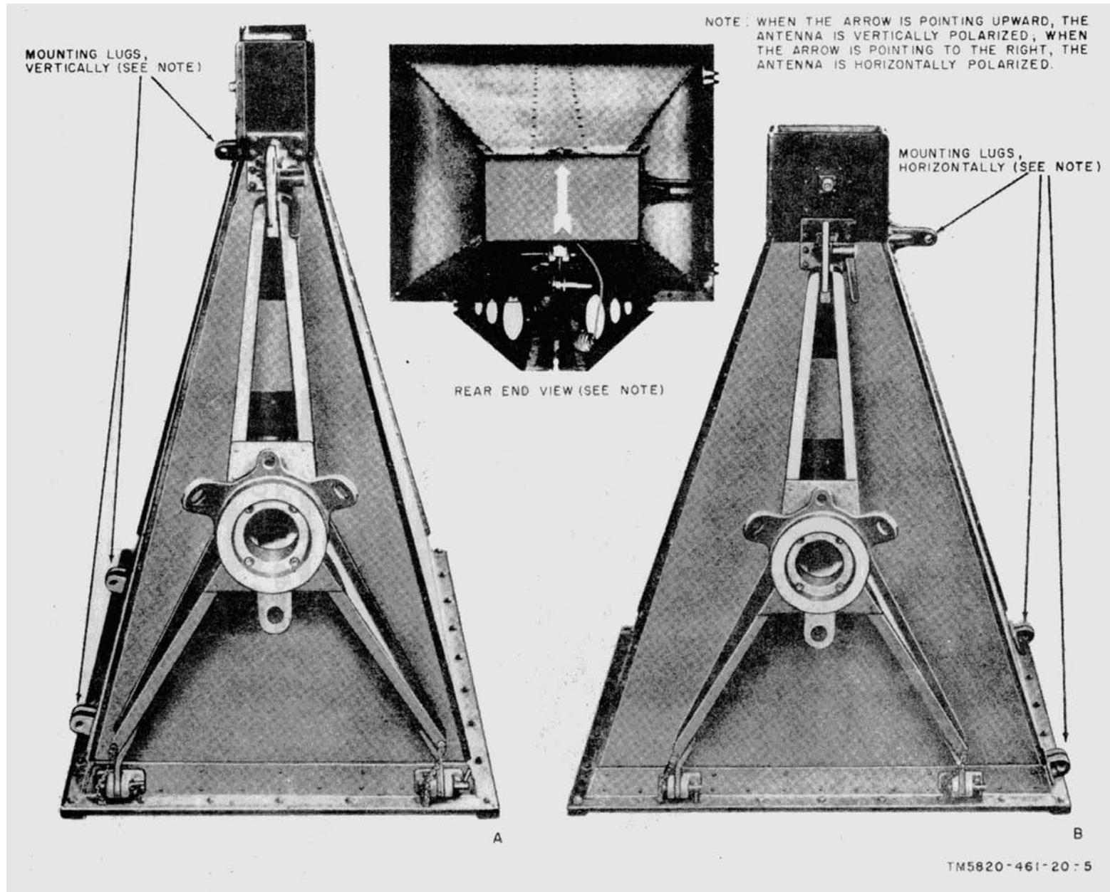
Figure 1-7. Antenna AT-903/G 1-9
